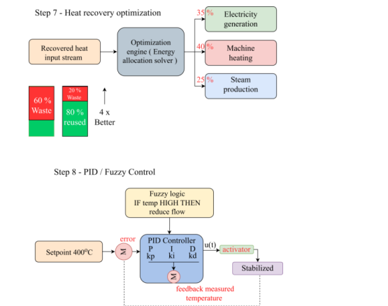
FIGURE 5: INTELLIGENT HEAT RECOVERY OPTIMIZATION AND HYBRID PID-FUZZY CONTROL SYSTEM
