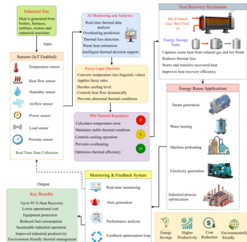
FIGURE 1: HYTHERM-OPT INDUSTRIAL HEAT RECOVERY FRAMEWORK
