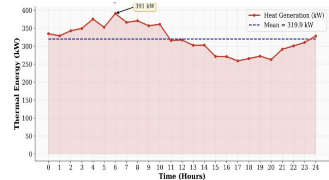
FIGURE 7: HEAT GENERATION TREND OVER TIME
